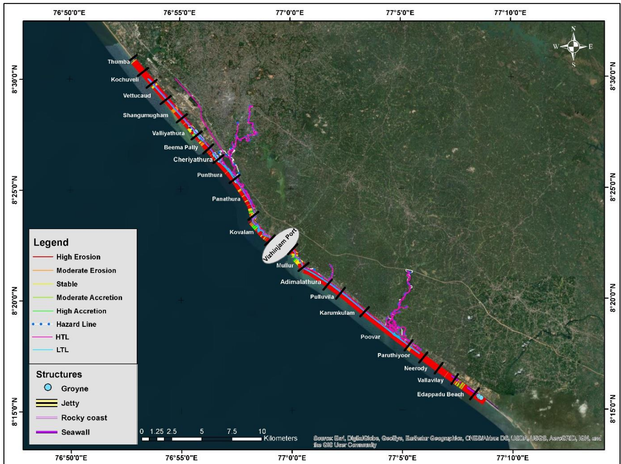
Figure 4.31 Shoreline Change Map – Fair Weather Period 2019
