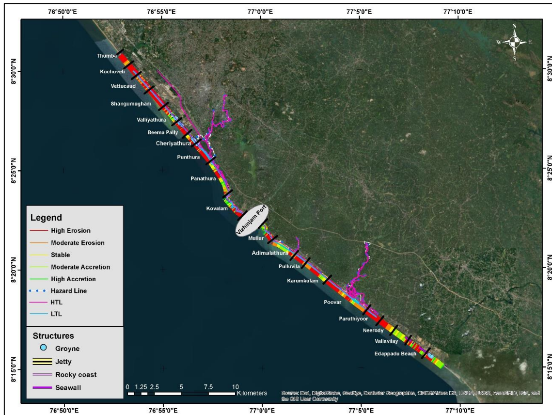
Figure 4.25 Shoreline Change Map - May 2019
