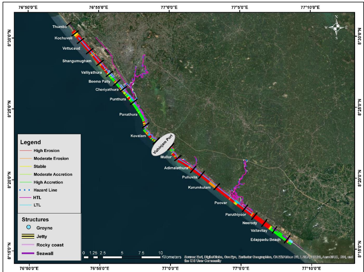
Figure 4.35 Shoreline Change Map October 2017 and October 2018
