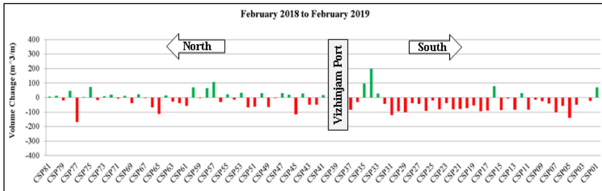
Figure 4.14 Beach Volume Changes - February 2018 and February 2019 in m^3/m
