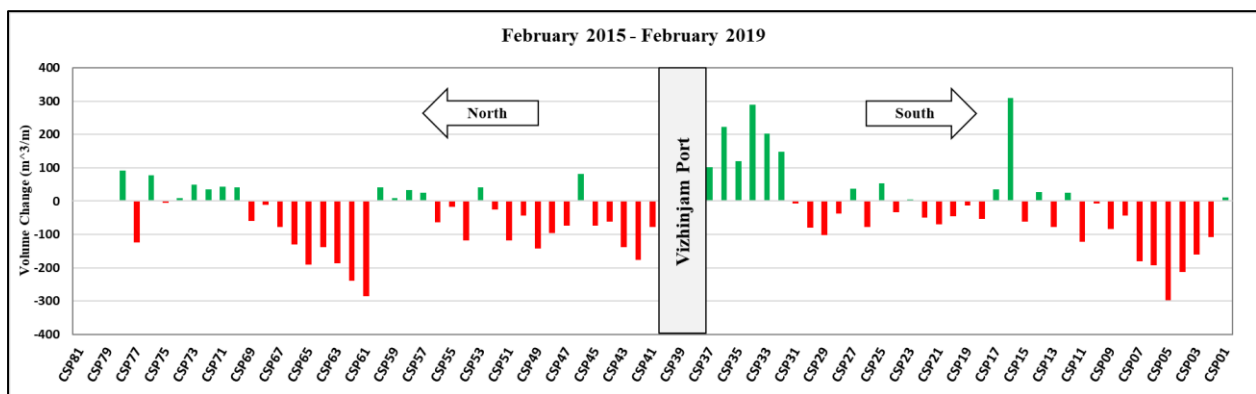
Figure 4.17 Beach Volume Changes - February 2015 and February 2019 in m 3 /m
