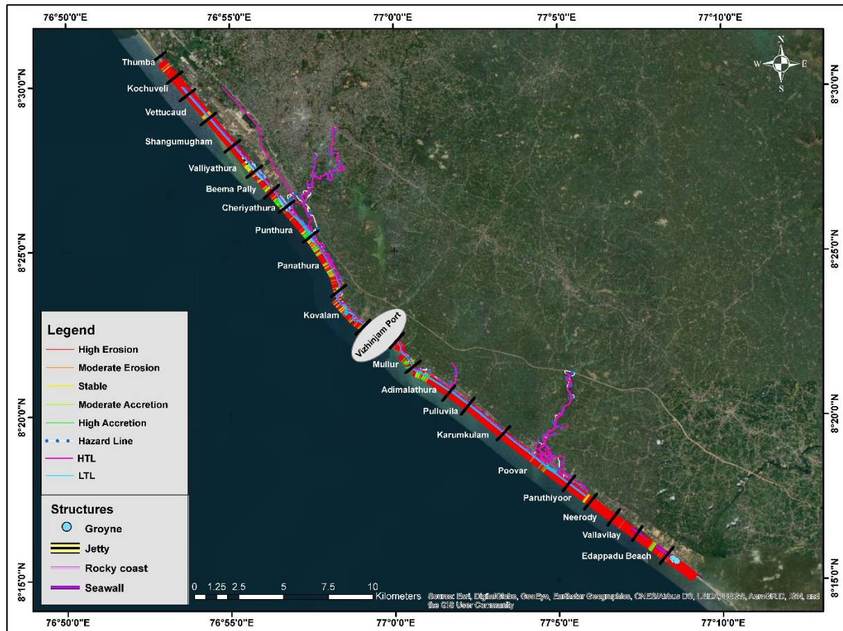
Figure 4.37 Shoreline Change Map September 2018 and September 2019
