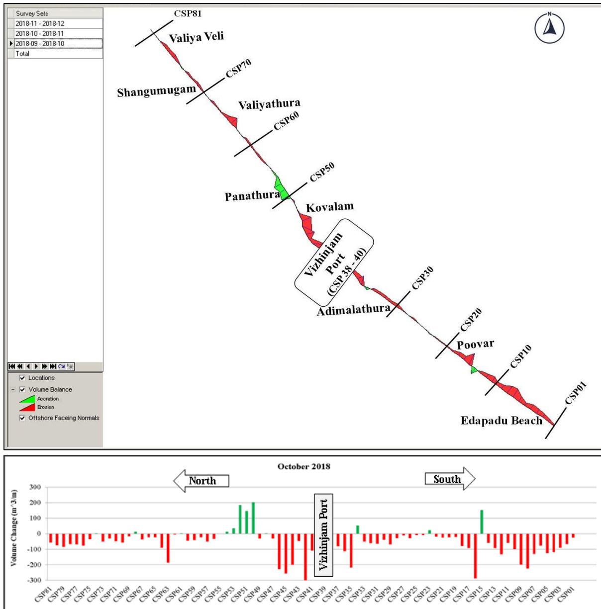
Figure 4.1 Monthly Beach Volume Changes in October 2018 in m^3/m
