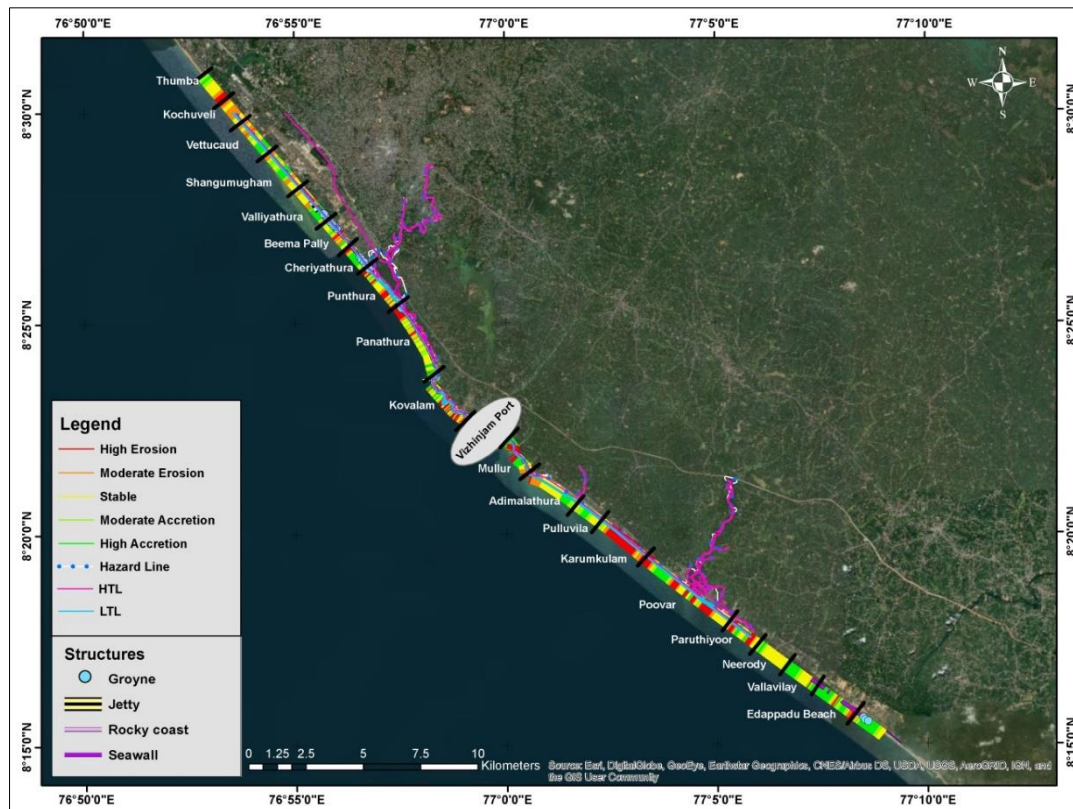
Figure 4.27 Shoreline Change Map – July 2019
