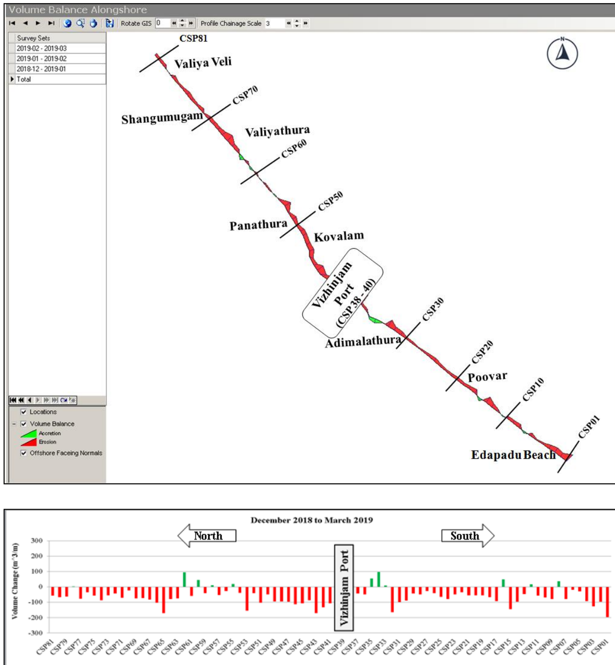
Figure 4.10 Seasonal Beach Volume Changes during Fair weather period in m^3/m
