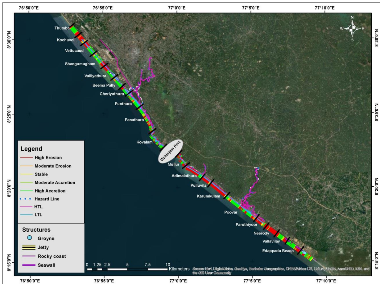
Figure 4.33 Shoreline Change Map – Monsoon Period 2019
