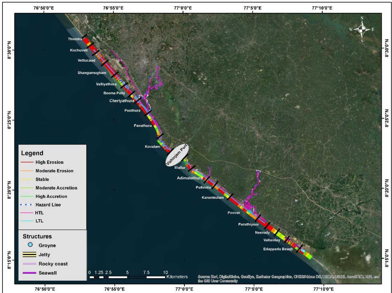
Figure 4.32 Shoreline Change Map – Pre-Monsoon Period 2019
