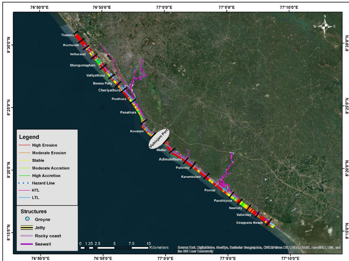
Figure 4.23 Shoreline Change Map - March 2019
