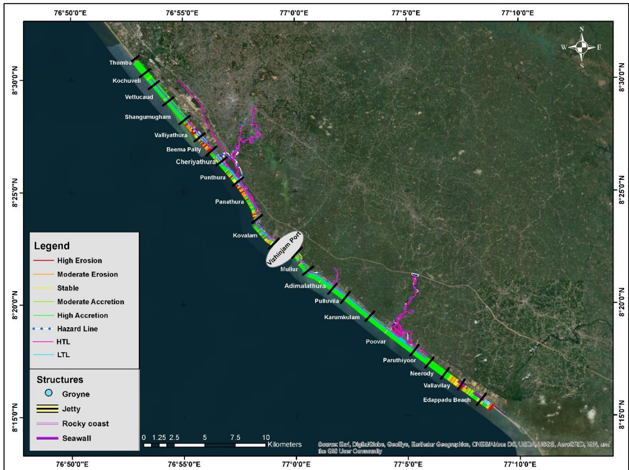
Figure 4.30 Shoreline Change Map – Post Monsoon 2018
