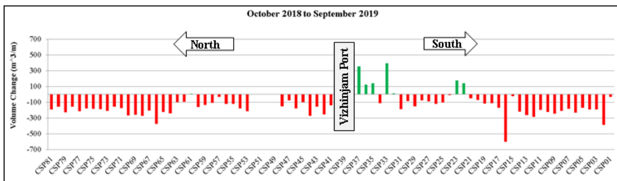
Figure 4.12 Overall Beach Volume Changes - October 2018 to September 2019 in m 3 /m
