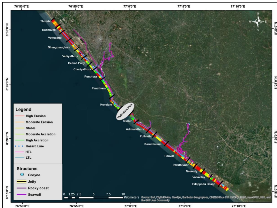
Figure 4.28 Shoreline Change Map - August 2019
