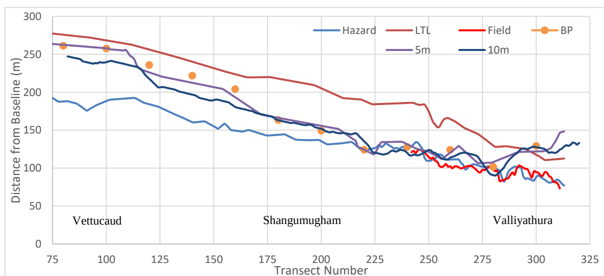
Figure 4.40 Comparison of Shoreline data from satellite images of different spatial resolution, beach profile data, LTL, Hazard line with field shoreline from Vettucaud to Valliyathura
