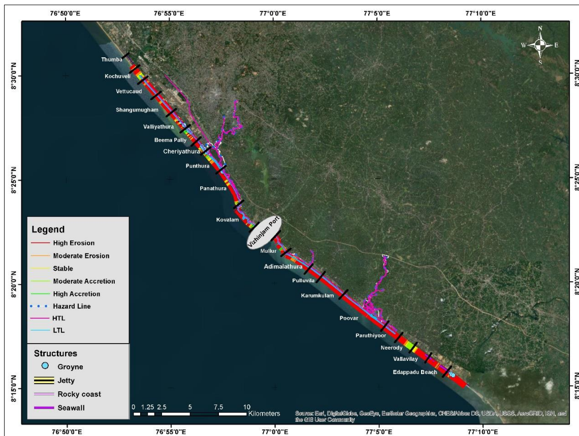
Figure 4.24 Shoreline Change Map - April 2019
