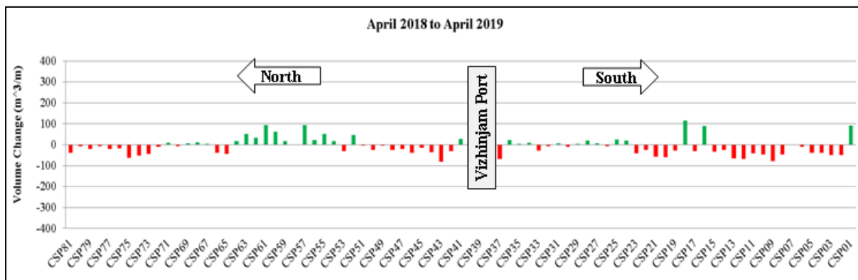
Figure 4.15 Beach Volume Changes - April 2018 and April 2019 in m^3/m
