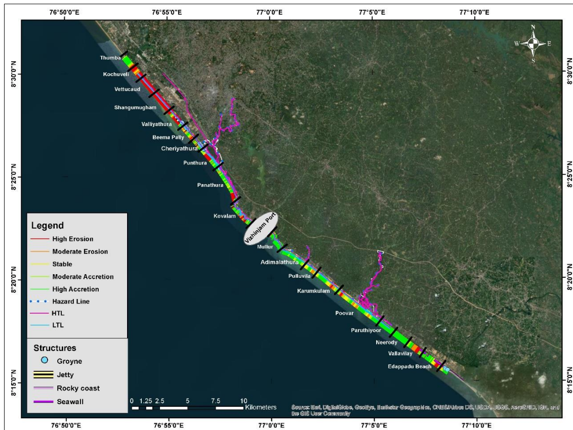
Figure 4.21 Shoreline Change Map - January 2019
