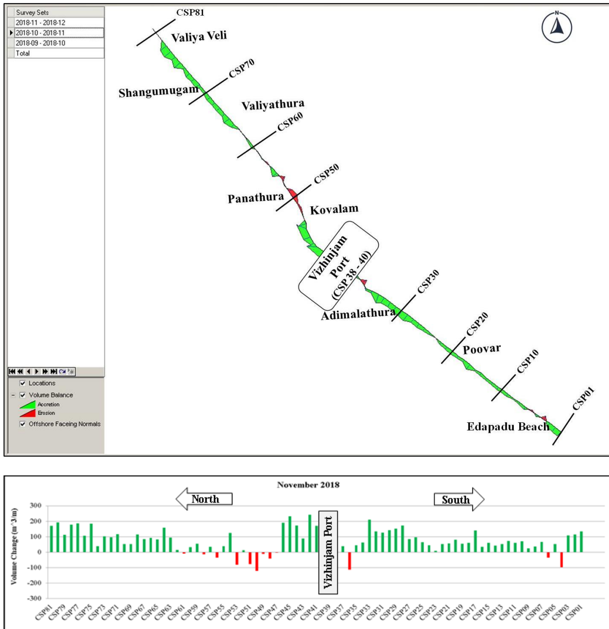
Figure 4.2 Monthly Beach Volume Changes in November 2018 in m^3/m
