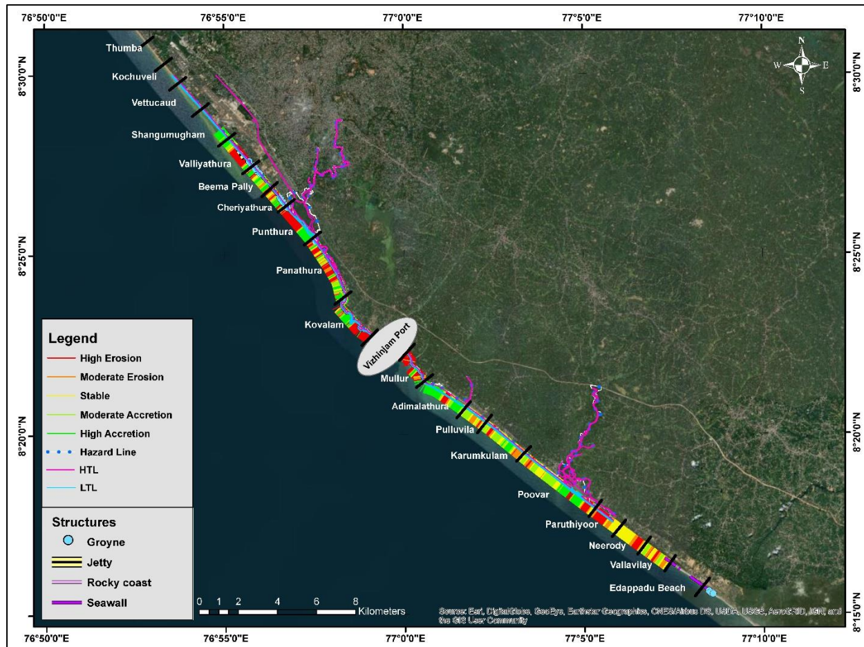
Figure 4.36 Shoreline Change Map February 2018 and February 2019
