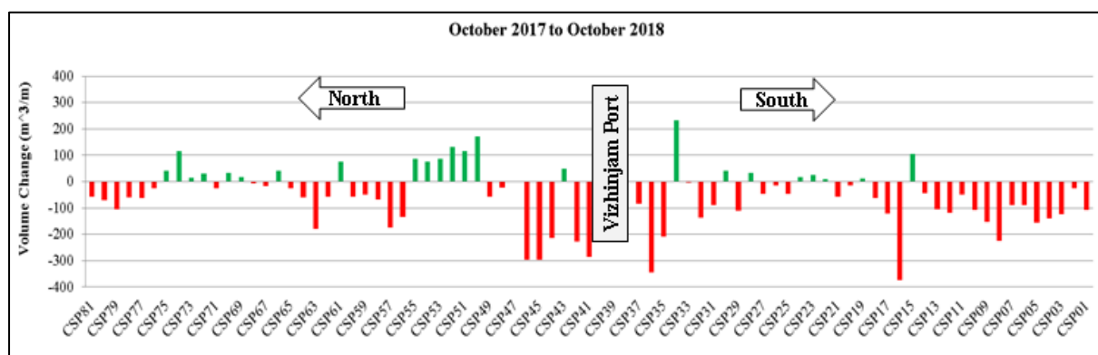
Figure 4.13 Beach Volume Changes - October 2017 and October 2018 in m³/m
