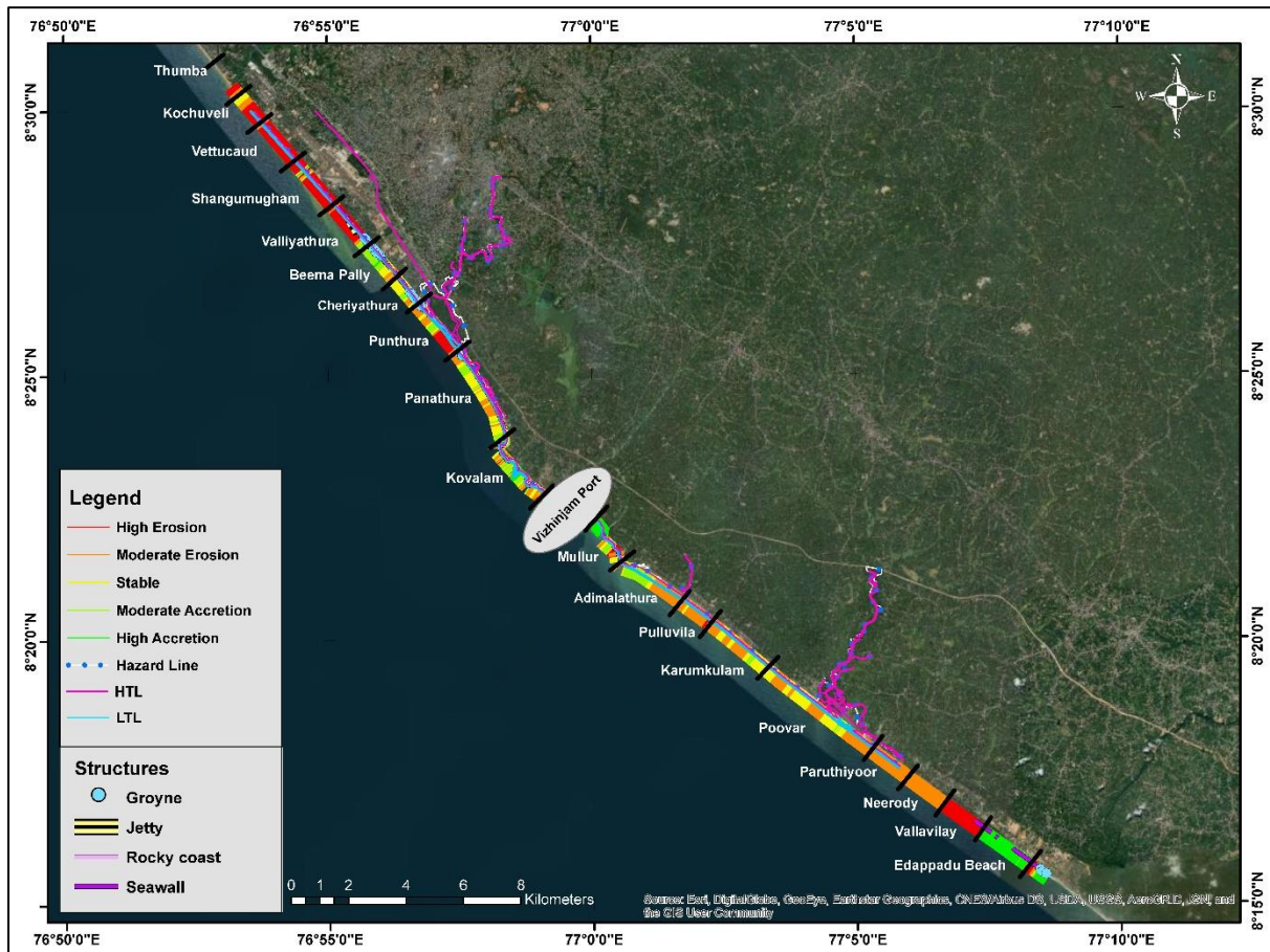
Figure 4.38 Shoreline Change Map- January 2015 to February 2019
