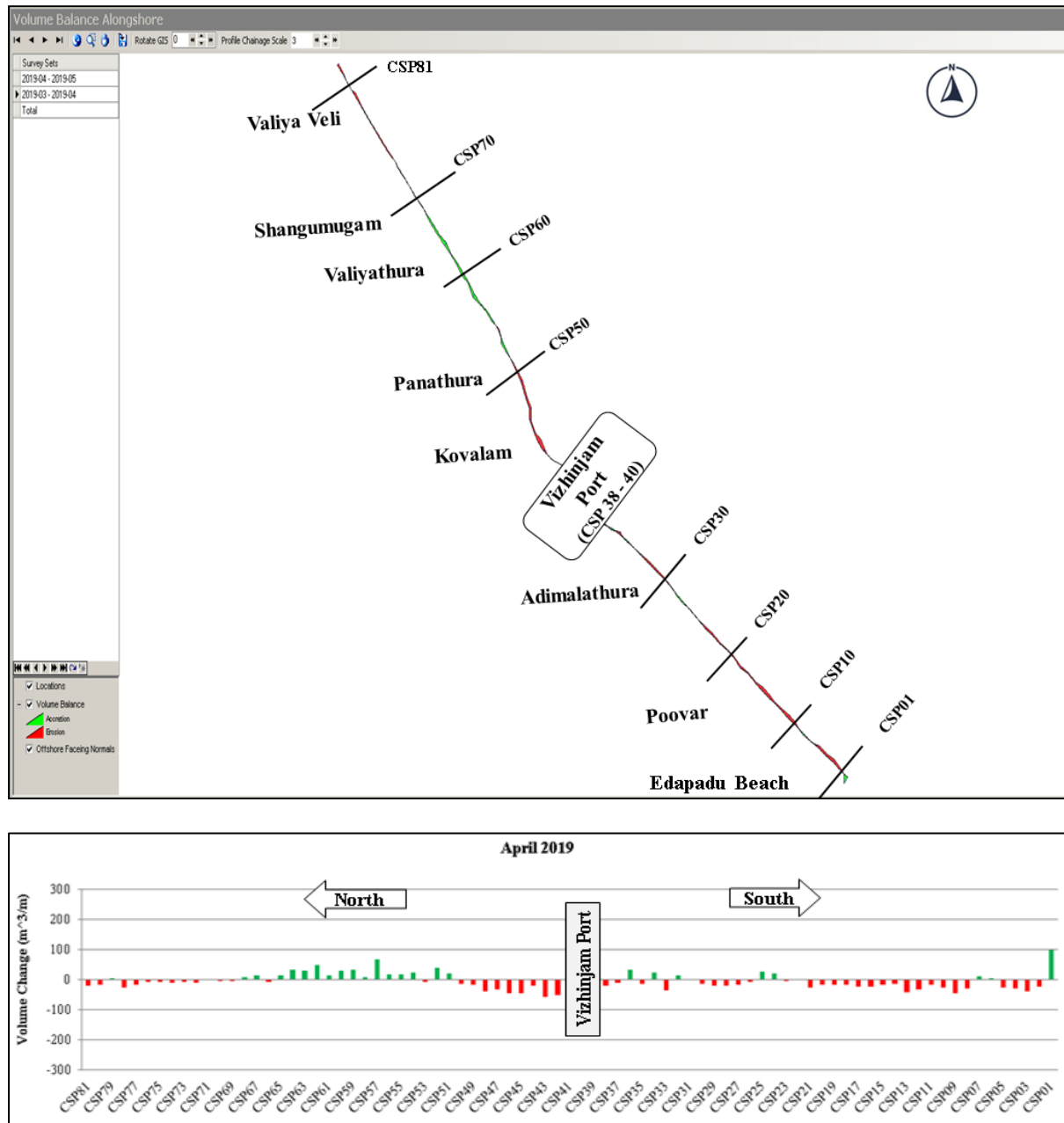
Figure 4.7 Monthly Beach Volume Changes in April 2019 in m^3/m
