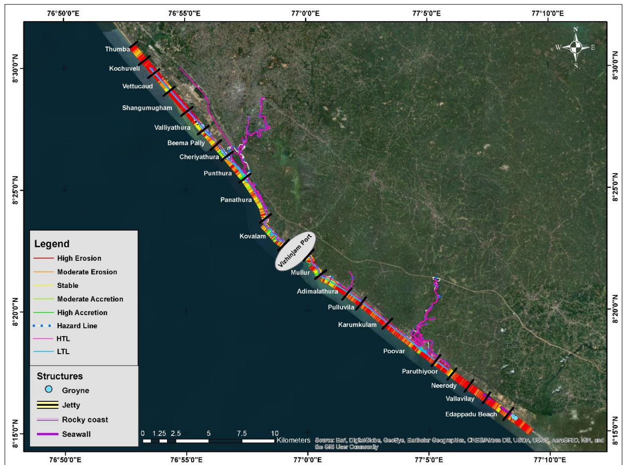
Figure 4.34 Overall Shoreline Change Map October 2018 to September 2019
