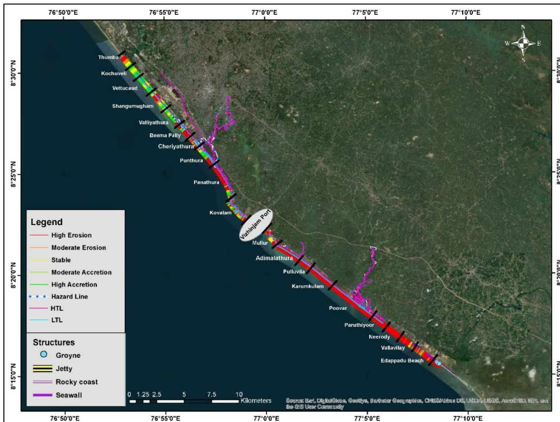
Figure 4.22 Shoreline Change Map - February 2019
