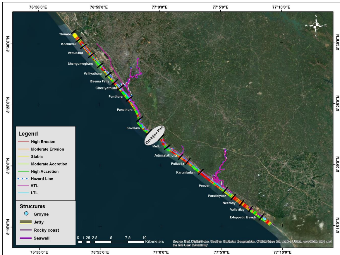
Figure 4.18 Shoreline Change Map - October 2018
