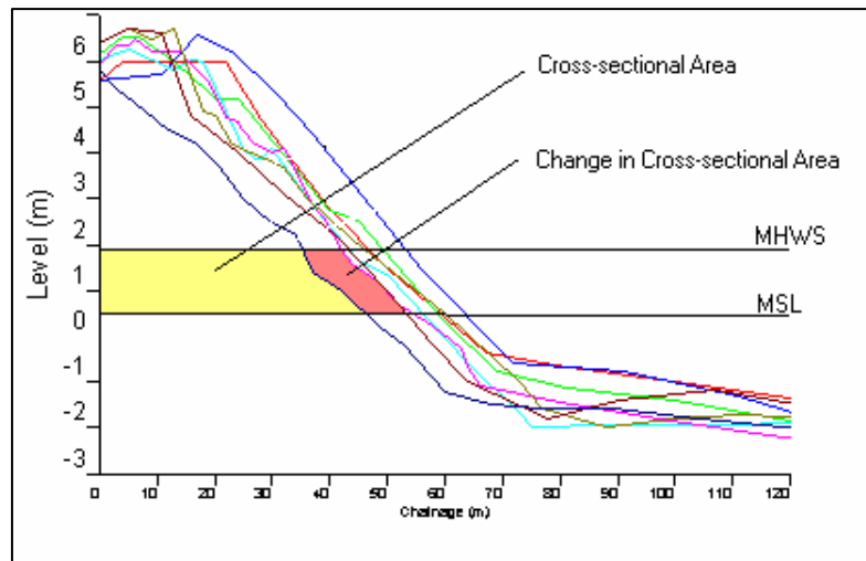
Figure 3.7 Profile Analysis by Level
