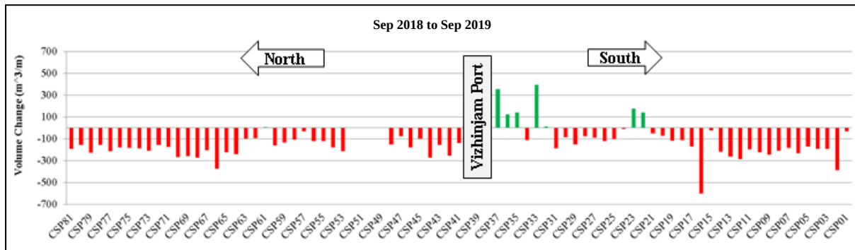
Figure 4.16 Beach Volume Changes - September 2018 and September 2019 in m 3 /m
