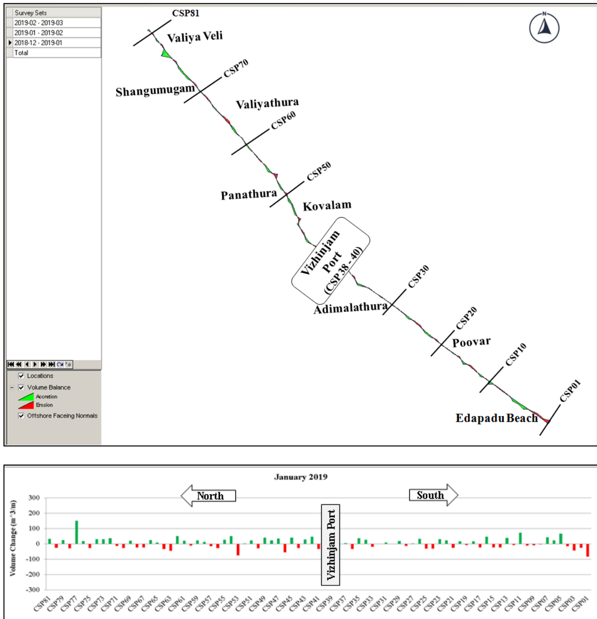
Figure 4.4 Monthly Beach Volume Changes in January 2019 in m^3/m
