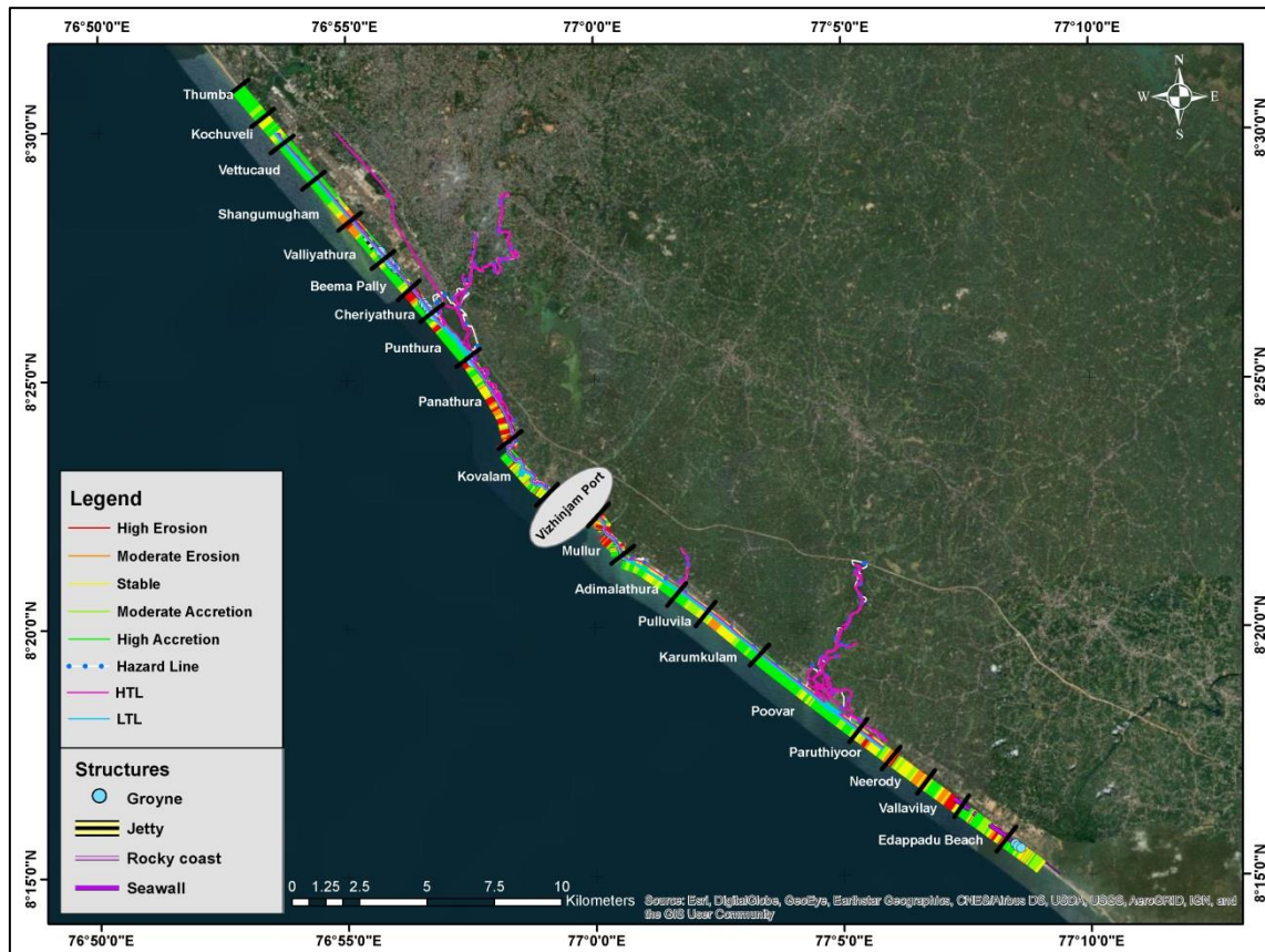
Figure 4.29 Shoreline Change Map - September 2019
