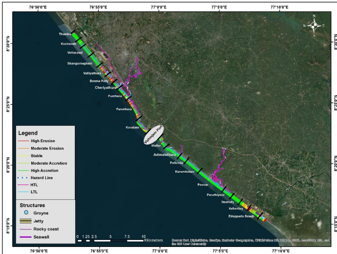
Figure 4.19 Shoreline Change Map - November 2018
