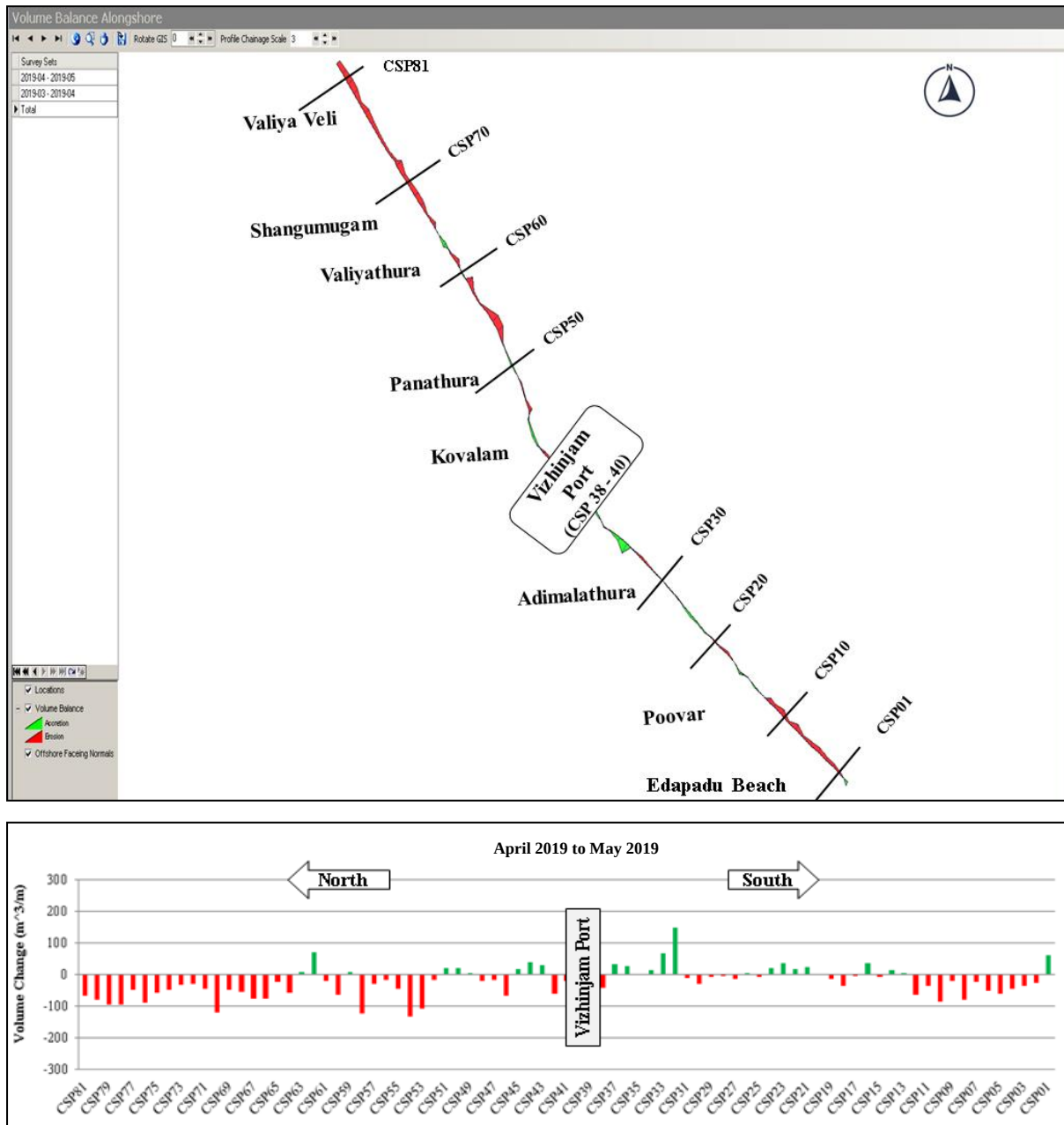
Figure 4.11 Seasonal Beach Volume Changes during Pre-Monsoon Period 2019 in m³/m
