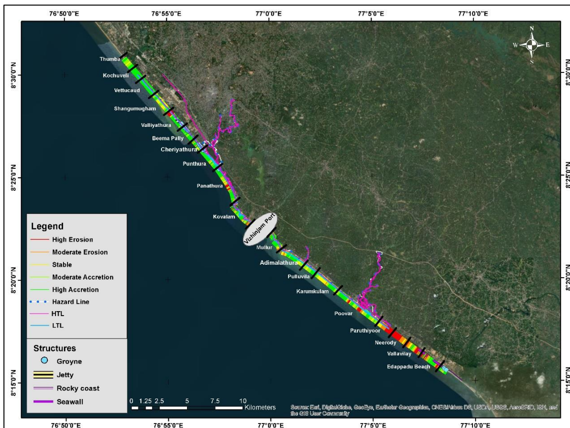
Figure 4.20 Shoreline Change Map - December 2018
