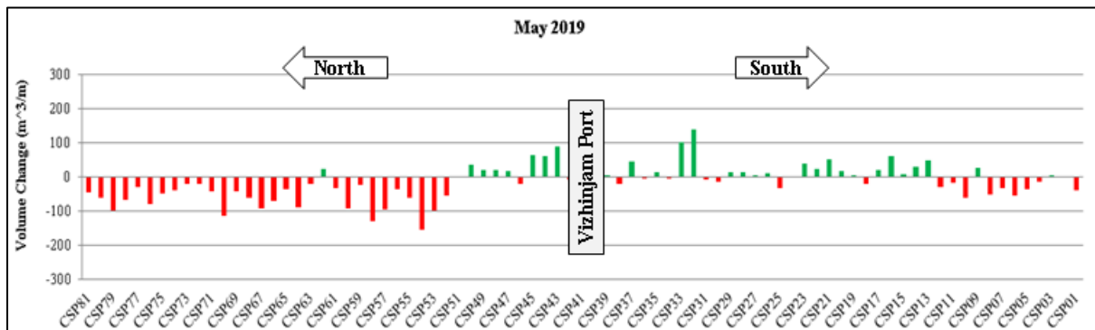
Figure 4.8 Monthly Beach Volume Changes in May 2019 in m 3 /m
