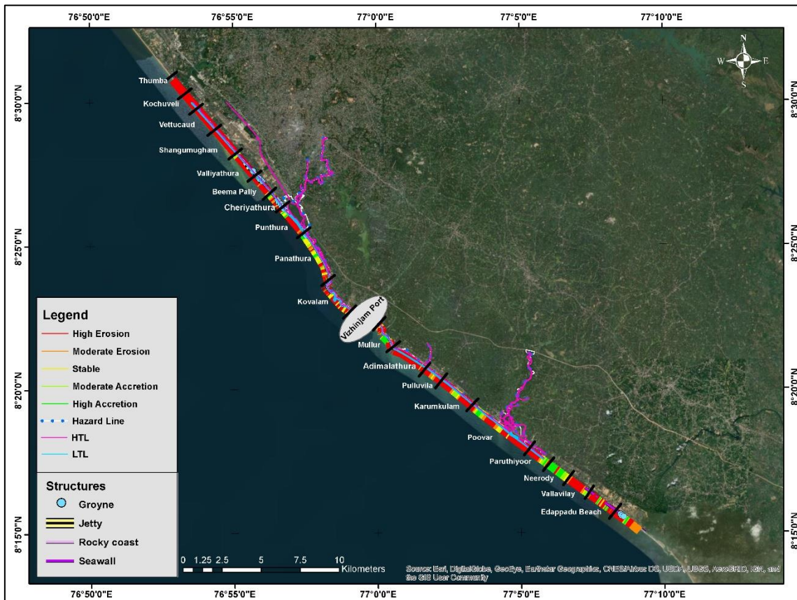
Figure 4.26 Shoreline Change Map - June 2019
