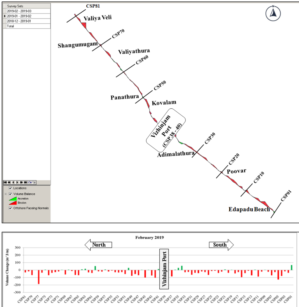
Figure 4.5 Monthly Beach Volume Changes in February 2019 in m^3/m
