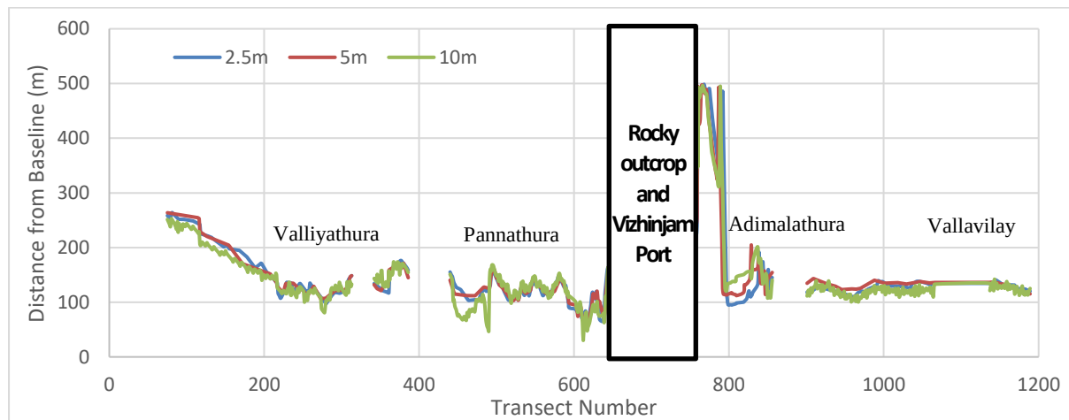
Figure 4.39 Comparison of Shoreline data from satellite images of different spatial resolution and beach profile data with field shoreline
